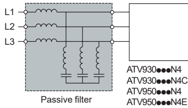
Passive filter Altivar Process drive with passive filter
